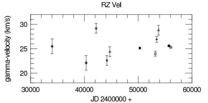
Figure 9. \gamma -velocities of RZ Velorum. The symbols for the different data sets are the same as in Fig. 8.
