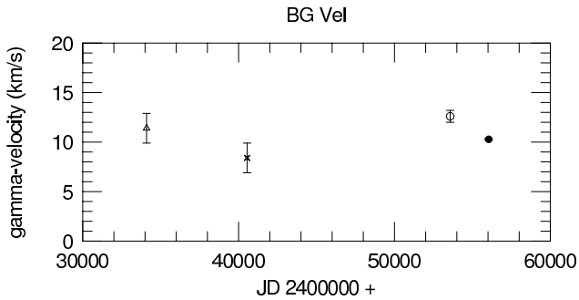
Figure 13. \gamma -velocities of BG Velorum. The symbols for the different data sets are the same as in Fig. 12.
