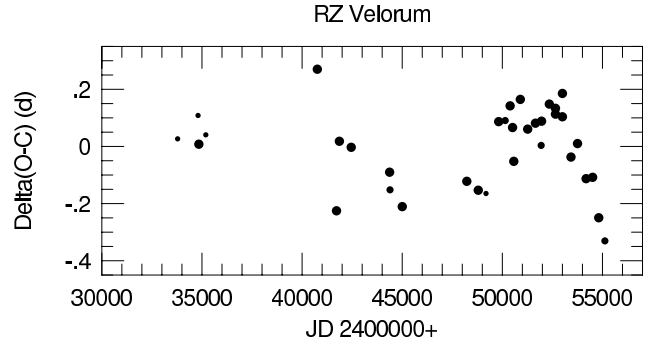
Figure 7. \Delta(O - C) diagram of RZ Vel.
