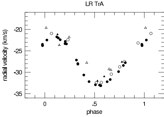
Figure 4. Merged RV phase curve of LR TrA. Different symbols mean data from different years: 2005: filled triangles; 2006: empty triangles; 2007: triangular star; 2012: filled circles; 2013: empty circles. Zero phase was arbitrarily chosen at JD 2400 000.0 (in all merged RV phase curves in this paper).
