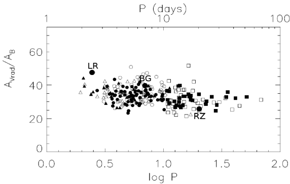
Figure 14. The slightly excessive value of the A_{VRAD}/A_B amplitude ratio of LR TrA and BG Vel (large circles) with respect to the average value characteristic at the given pulsation period is an independent indication of the presence of a companion star. This is a modified version of Fig. 4f of Klagyivik & Szabados (2009). For the meaning of various symbols, see the original figure.
