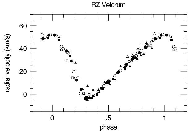
Figure 8. Radial velocity phase curve of RZ Vel. Data obtained between 1996 and 2013 are included in this plot. The meaning of various symbols is explained in the text.
